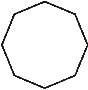
Regular Octagon S=8 V=8
